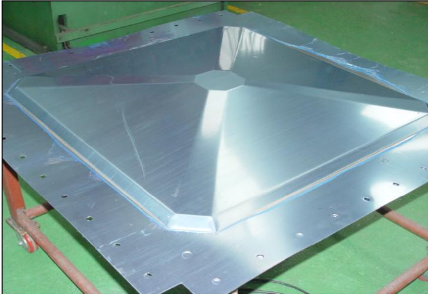
Hole Cutting of Assembly Part
